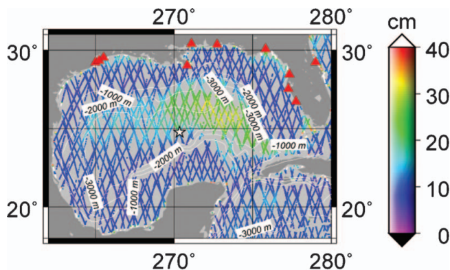
Figure 3. Standard deviations of residual SSH anomaly at along satellite track locations and location of tide gauge sites used as the ground truth (pelagic sites shown as stars and coastal sites as triangles) with contour indicating the depth of ocean (positive upward in meters) in the Gulf of Mexico region. (Figure appears in color online.)
