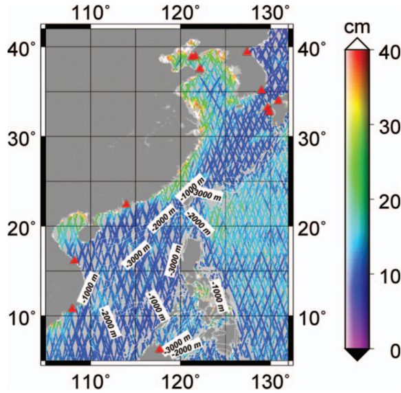
Figure 5. Standard deviations of residual SSH anomaly at along satellite track locations and location of tide gauge sites used as the ground truth (pelagic sites shown as stars and coastal sites as triangles) with contour indicating the depth of ocean (positive upward in meters) in Southeast China region. (Figure appears in color online.)
