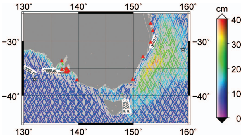
Figure 6. Standard deviations of residual SSH anomaly at along satellite track locations and location of tide gauge sites used as the ground truth (pelagic sites shown as stars and coastal sites as triangles) with contour indicating the depth of ocean (positive upward in meters) in East Australia region. (Figure appears in color online.)
