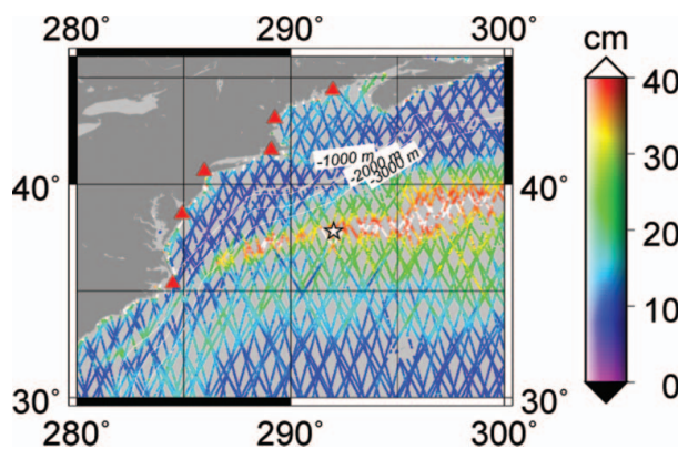
Figure 2. Standard deviations of residual SSH anomaly at along satellite track locations and location of tide gauge sites used as the ground truth (pelagic sites shown as stars and coastal sites as triangles) with contour indicating the depth of ocean (positive upward in meters) in the Northwest Atlantic region. (Figure appears in color online.)
