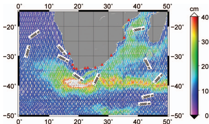
Figure 7. Standard deviations of residual SSH anomaly at along satellite track locations and location of tide gauge sites used as the ground truth (pelagic sites shown as stars and coastal sites as triangles) with contour indicating the depth of ocean (positive upward in meters) in South Africa region. (Figure appears in color online.)
