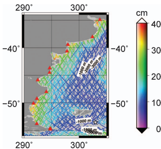
Figure 4. Standard deviations of residual SSH anomaly at along satellite track locations and location of tide gauge sites used as the ground truth (pelagic sites shown as stars and coastal sites as triangles) with contour indicating the depth of ocean (positive upward in meters) in Patagonia Shelf region. (Figure appears in color online.)
